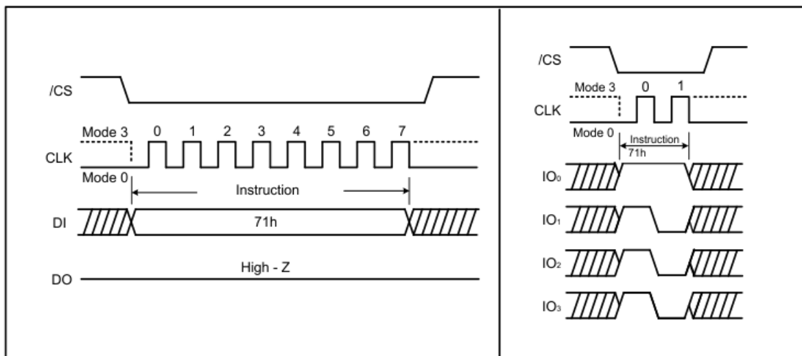
Figure 15 Clear Flag Status Register Sequence Diagram (SPI&QPI)
