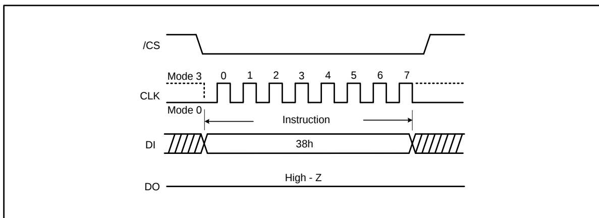
Figure 51. Enter QPI Instruction (SPI Mode only)
