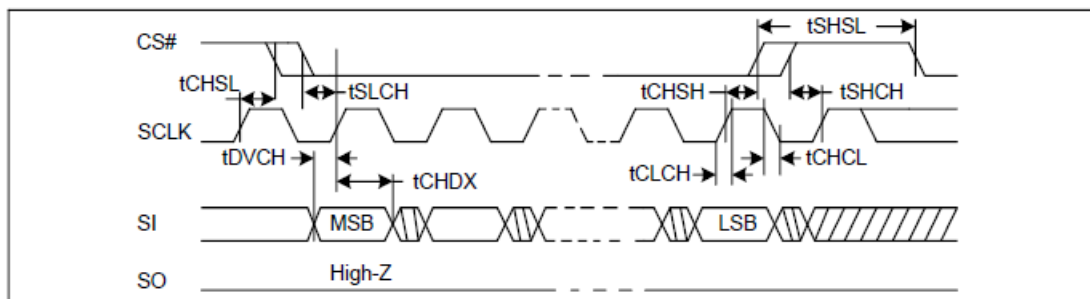
Figure 57. Input Timing
