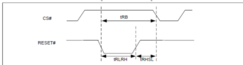
Figure 59. Reset Timing
