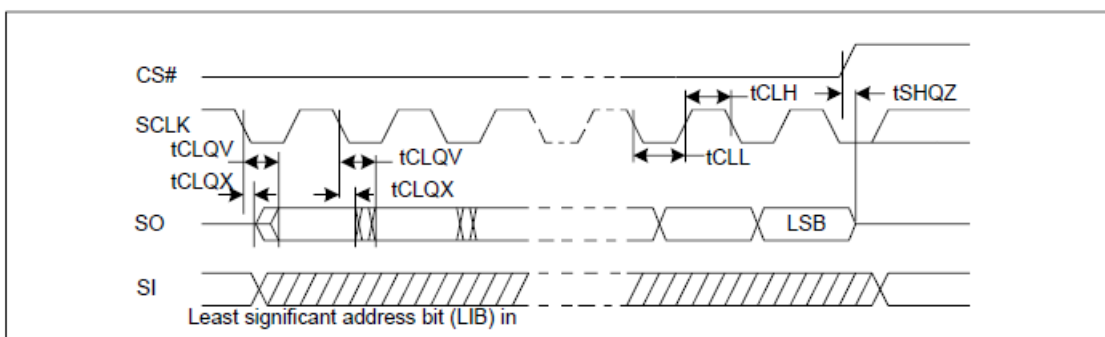
Figure 58. Output Timing
