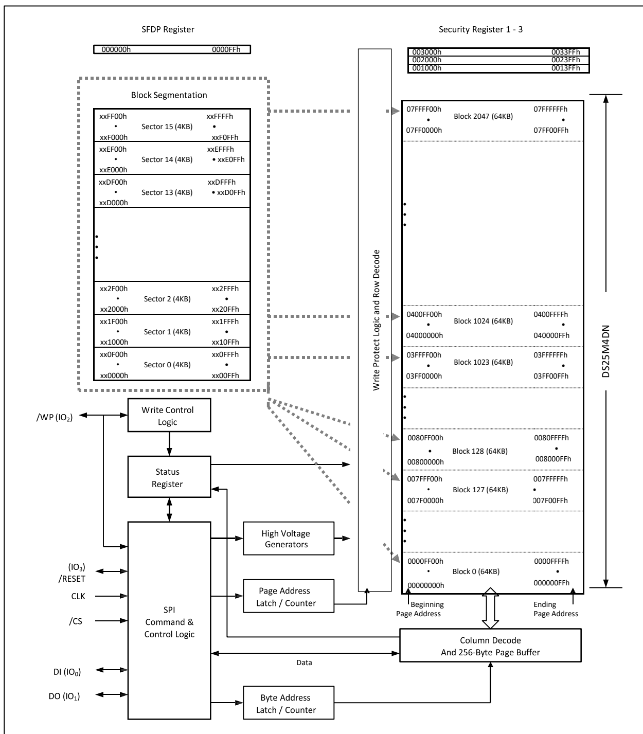
Figure 2. DS25M4DN Serial Flash Memory Block Diagram
