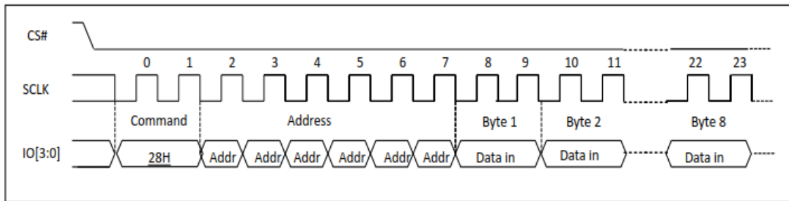
Figure 46b Write Password Sequence Diagram (QPI)
