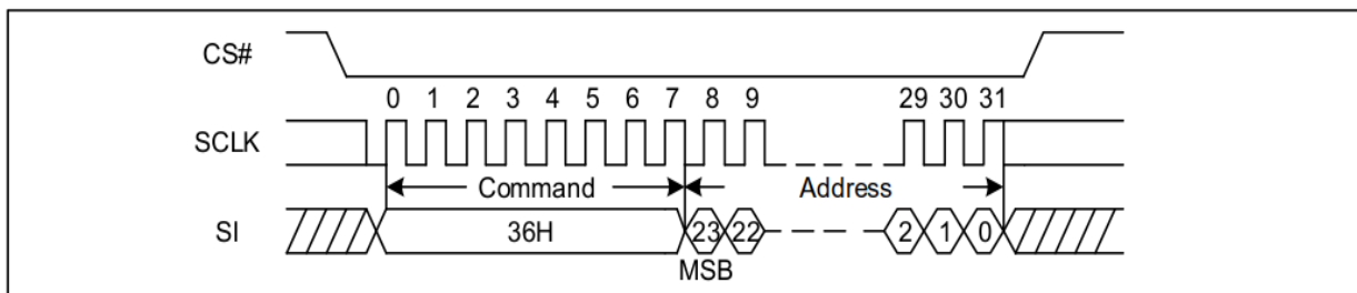
Figure 43a Individual Block/Sector Lock command Sequence Diagram (SPI)
