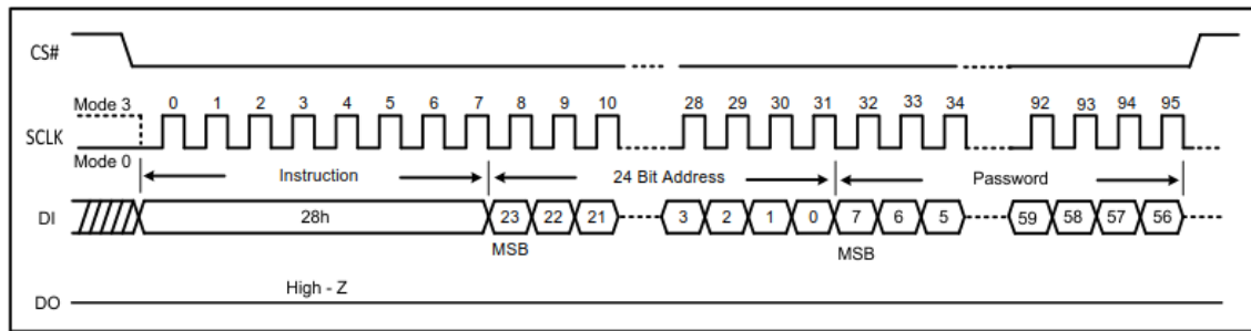
Figure 46a Write Password Sequence Diagram (SPI)
